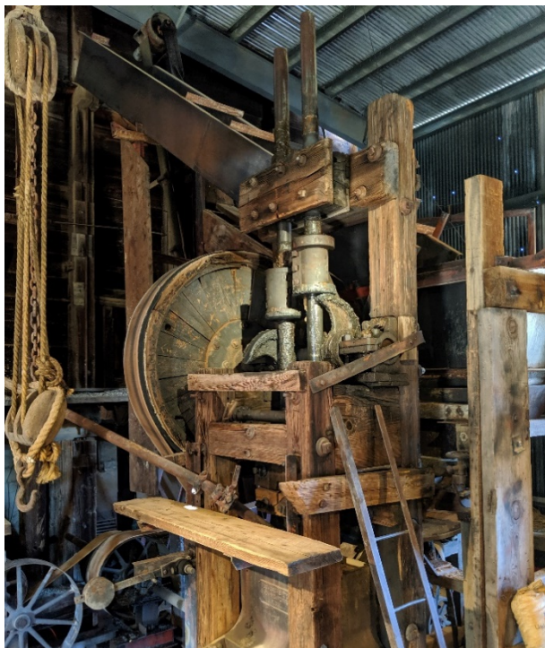
Figure 16. The current two-stamp mill at the Comstock mill.
